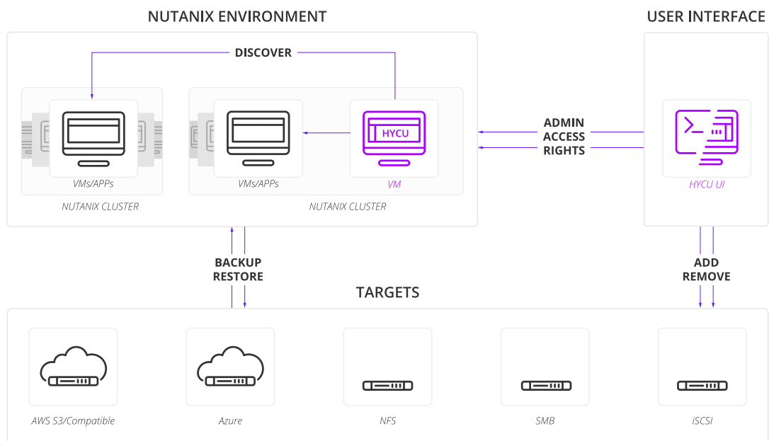
Figure 1-2: HYCU architecture
